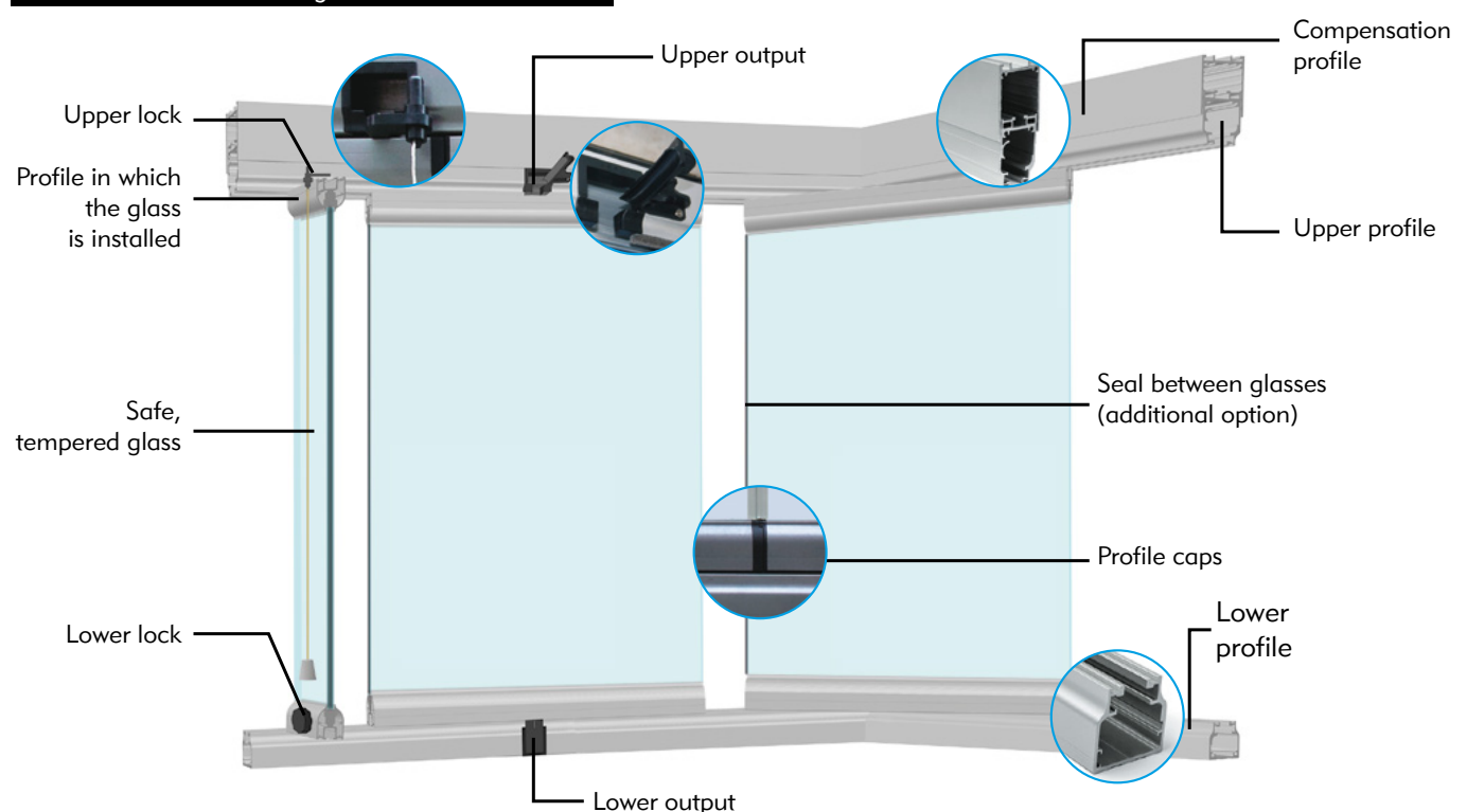
Schematic building frameless
